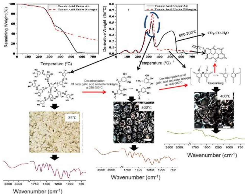
Figure 4: Diagram of the thermal behavior of polyphenolic tannin compound (20).
